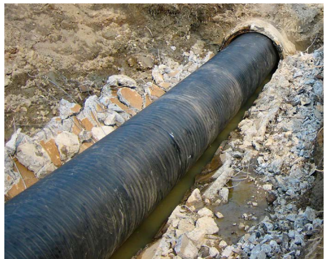
Hämeenlinna, Finland: A highway crossing was renovated by sliplining a Weholite pipe DN/ID 1000/1125mm into a concrete pipe DN 1300mm. Jointing type: Extrusion welding. Total length 750m.
